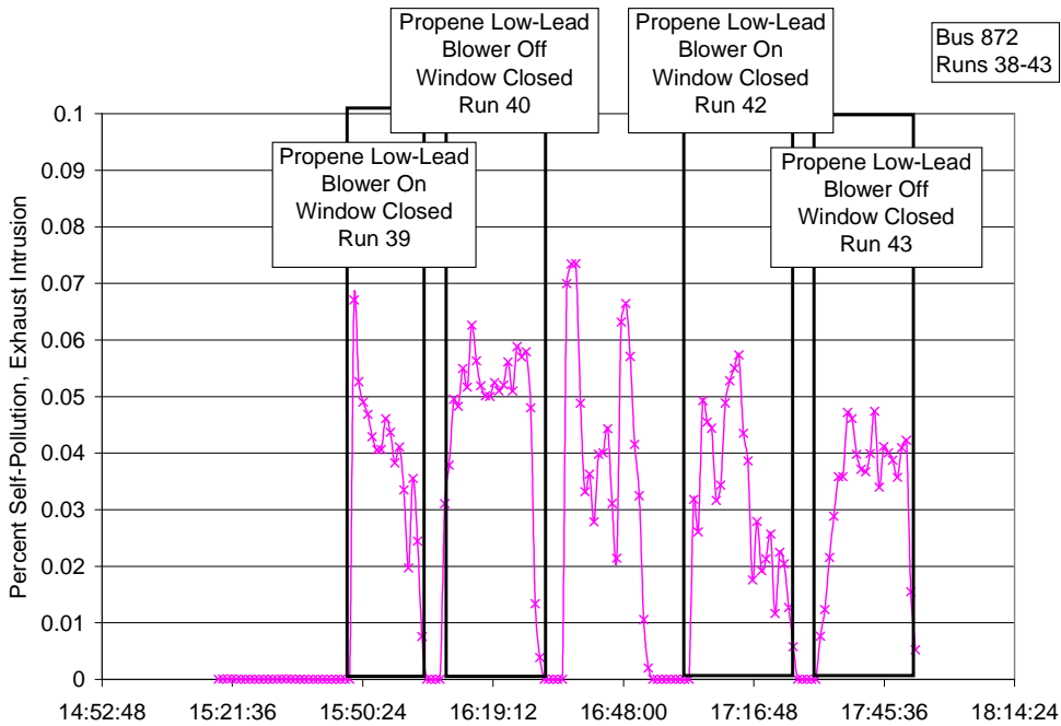
Figure 5.5.2 Time series of percent self-pollution and exhaust intrusion for propene during a leader exhaust-follower exhaust test on 0420.
