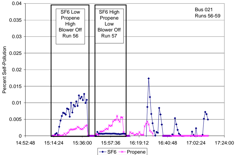
Figure 5.4.1.1.1 (b) Time series of percent self-pollution for SF 6 and propene during mobile runs conducted on 0504.
