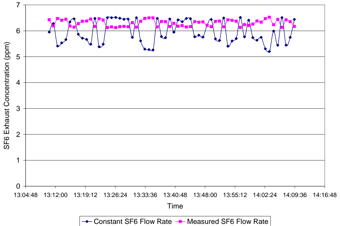
Figure 5.7.1. SF 6 tracer gas exhaust concentrations (1-minute medians) for Bus 982/TO1 on run 0407 calculated using measured SF 6 and exhaust flow rates versus those calculated with constant 2 lpm SF 6 flow rate and measured exhaust flow rate.
