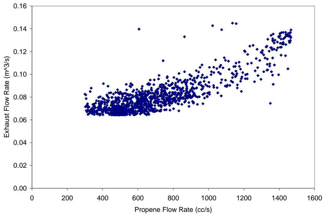
Figure 5.1.1.1.3 Scatter plots of exhaust flow versus propene flow rate for 0427/Run 44.
