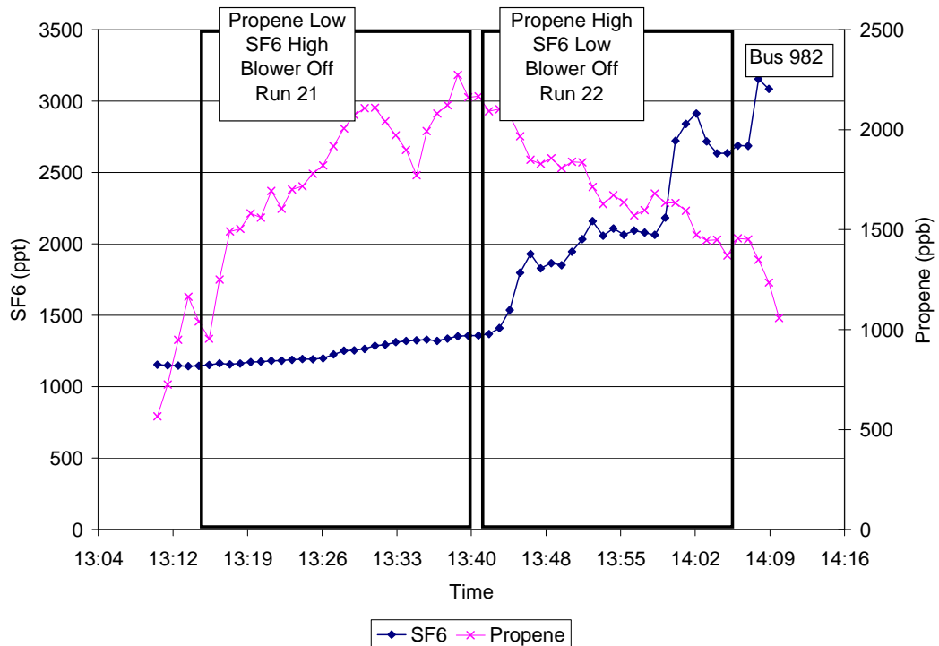
Figure 5.4.4.2 Time series for SF 6 and propene concentrations during window seal test on 0407 1 .
