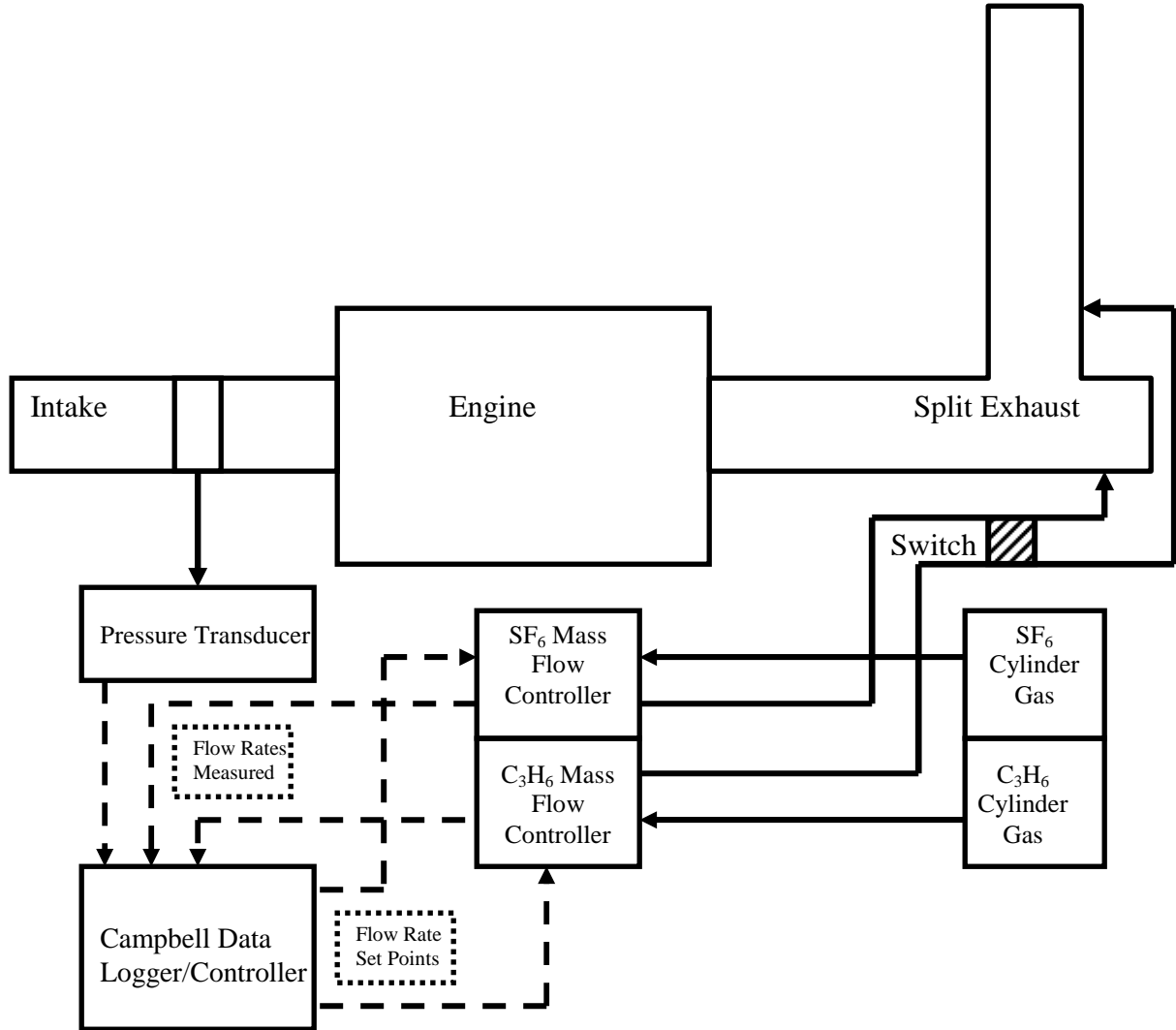
Figure 3.2.3.1 Tracer gas release system used in main study, using two tracer gases. The system was controlled by engine intake flow.
