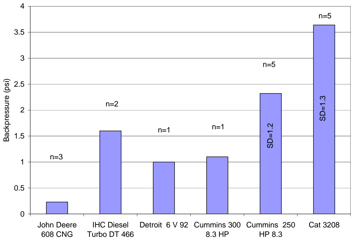
Figure 5.3.1 Backpressure measurements in psi for the six engine types tested in the exhaust leak experiment (n is the number of buses tested for each engine type). Standard deviations are provided for the Cummins 250 and Cat 3208 engines.
