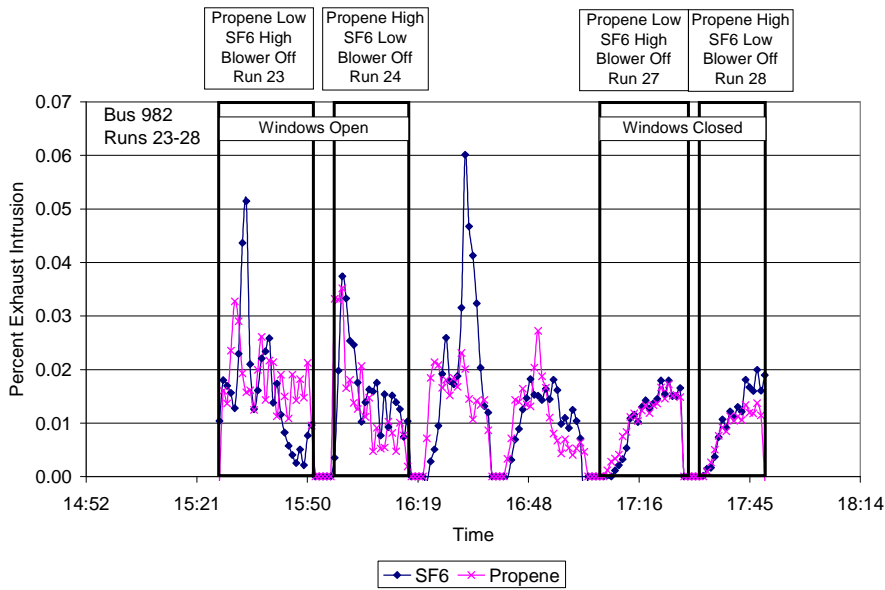
Figure 5.4.1.2.1 Time series for percent exhaust intrusion by SF 6 and propene on 0412 (leader exhaust test).
