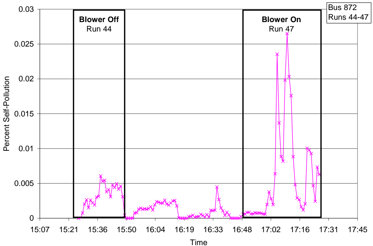
Figure 5.4.2.1.1 Time series for percent self-pollution by propene on 0427. The boxed areas represent runs where power ventilation was tested.
