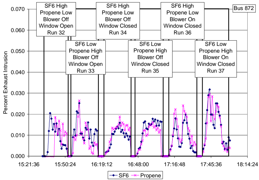
Figure 5.4.1.2.2 Time series for percent exhaust intrusion by SF 6 and propene on 0419 (leader exhaust test).
