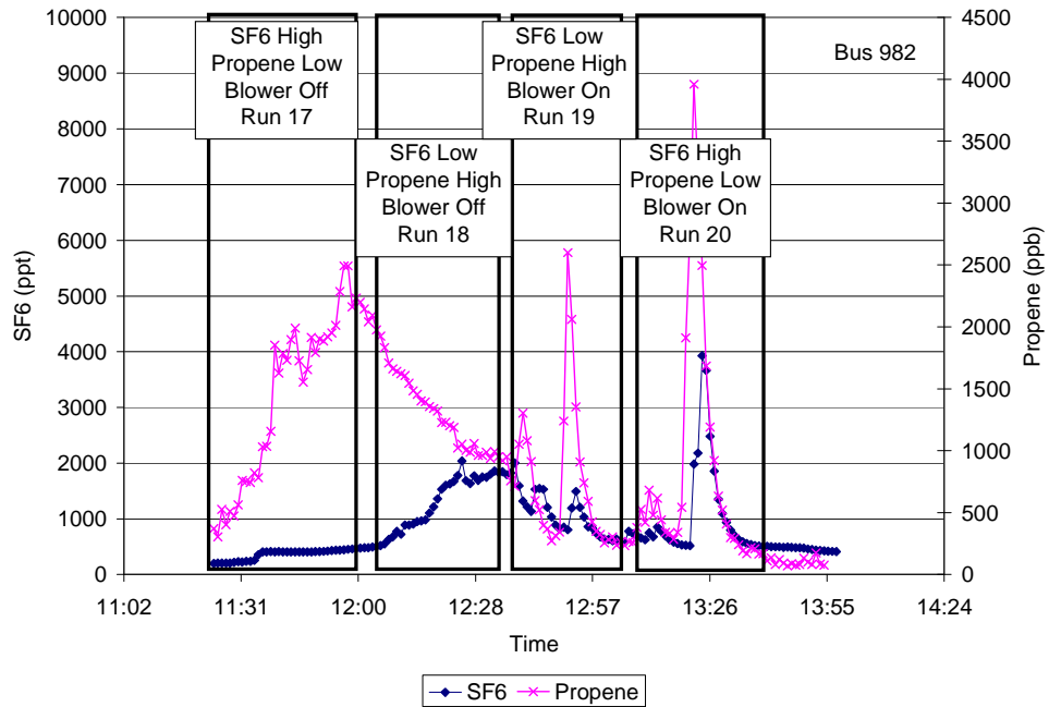
Figure 5.4.1.1.2 Time series for SF 6 and propene concentrations on 0406. The bus was not flushed of tracer gas for these runs.
