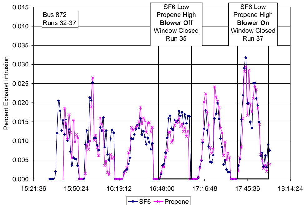
Figure 5.4.2.2.1 Time series for percent exhaust intrusion by SF 6 and propene on 0419 during a leader exhaust test. The boxed areas represent runs when power ventilation was tested.
