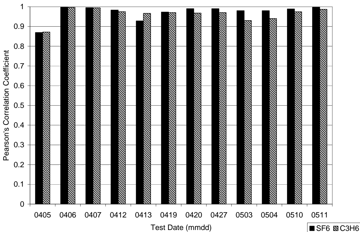
Figure 5.1.1.1.1 Pearson's correlation coefficient for each day of mobile testing in the main study.
