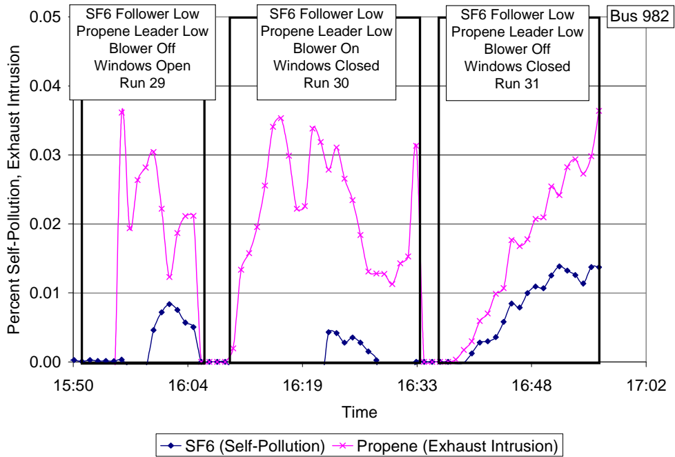
Figure 5.5.1 Time series of percent self-pollution and exhaust intrusion for SF 6 and propene, respectively, during a leader exhaust-follower exhaust test on 0413.
