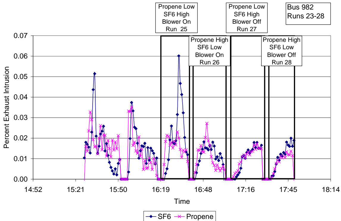
Figure 5.4.3.2.1 Time series of percent exhaust intrusion for SF 6 and propene during a leader exhaust run conducted on 0412.
