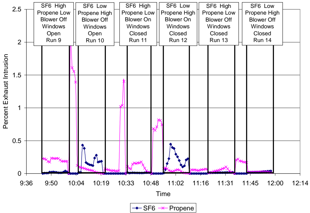
Figure 5.6.2.1 Time series for SF 6 and propene during stationary exhaust intrusion runs conducted on 0413.
