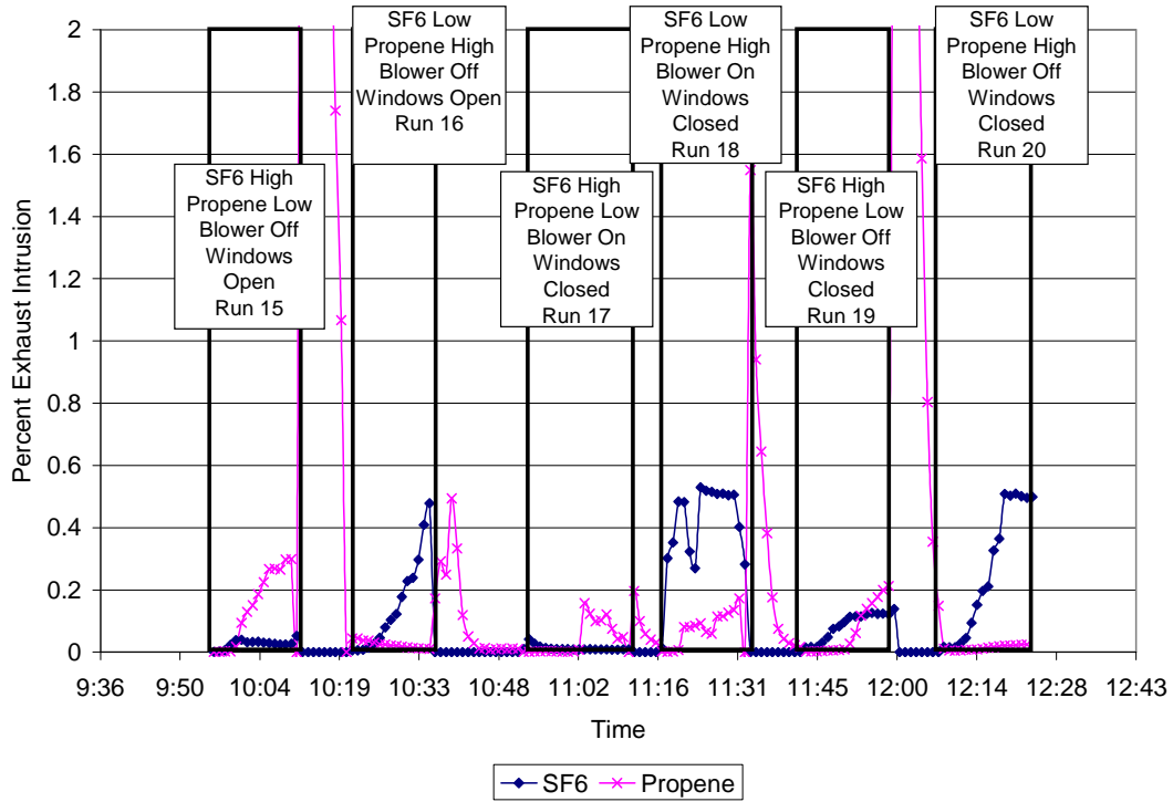
Figure 5.6.2.2 Time series for SF 6 and propene during stationary exhaust intrusion runs on 0420.
