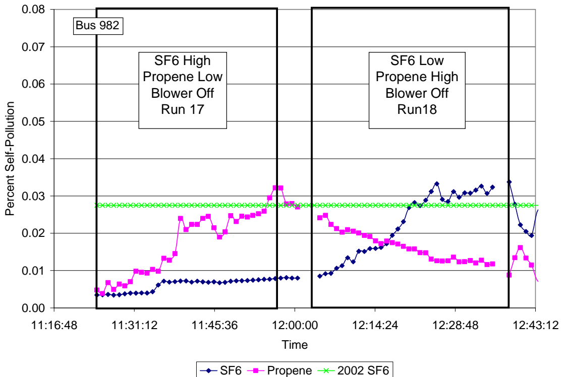
Figure 5.7.2 Time series for 0406 run in current study and average self-pollution value (0.0275%) from our previous study.
