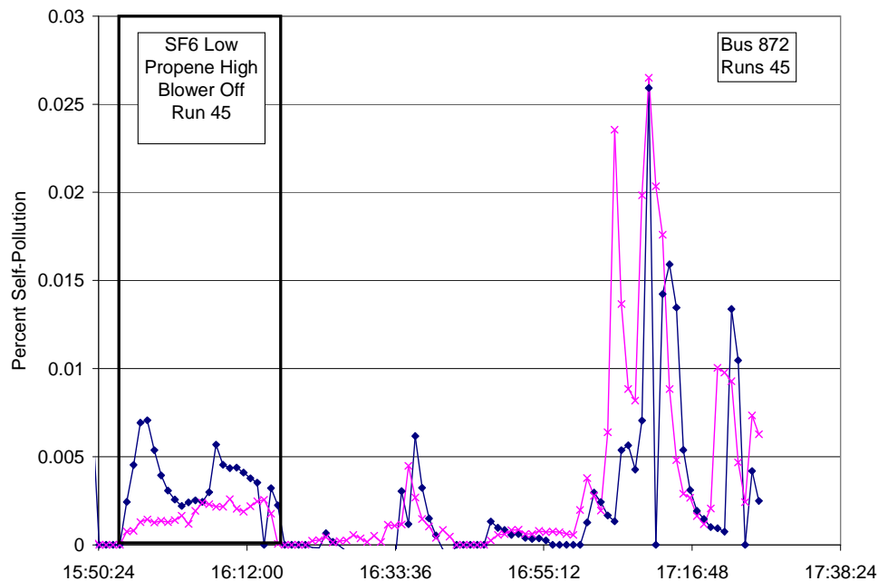
Figure 5.4.1.1.1 (a) Time series of percent self-pollution for SF 6 and propene during mobile runs conducted on 0427.
