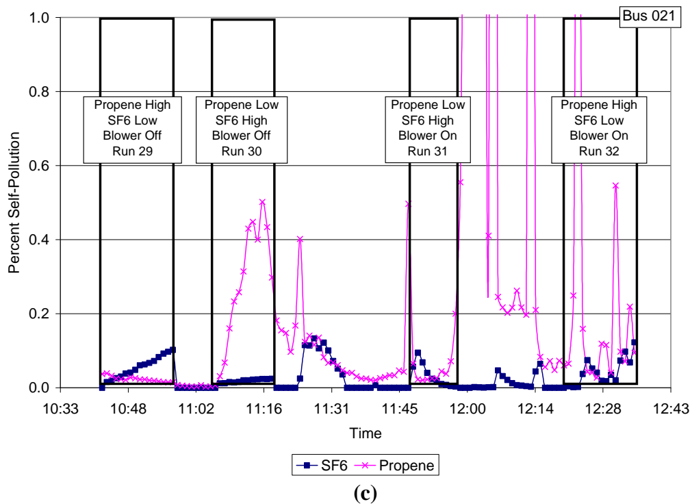
Figure 5.6.1.1 (c) Time series for SF 6 and propene during stationary self-pollution testing 0510.
