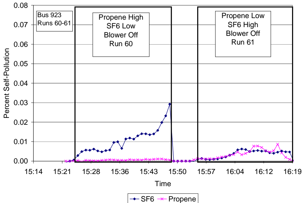
Figure 5.4.1.1.1 (c) Time series of percent self-pollution for SF 6 and propene during mobile runs conducted on 0510.
