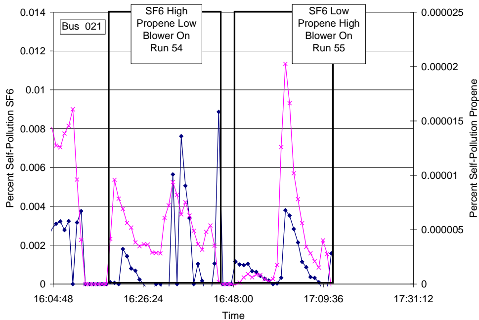
Figure 5.4.3.1.2 Time series of percent self-pollution for SF 6 and propene on 0503 examining the combination of exhaust position and blower operation as a mitigation measure.
