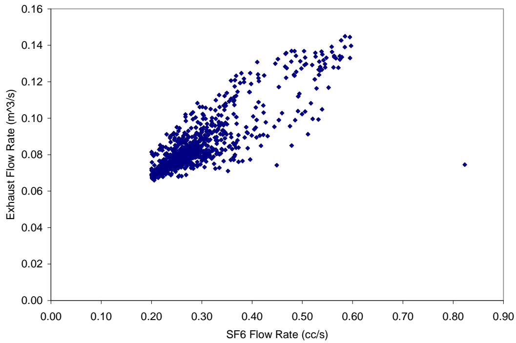
Figure 5.1.1.1.2 Scatter plots of exhaust flow versus SF 6 flow rate for 0427/Run 44.
