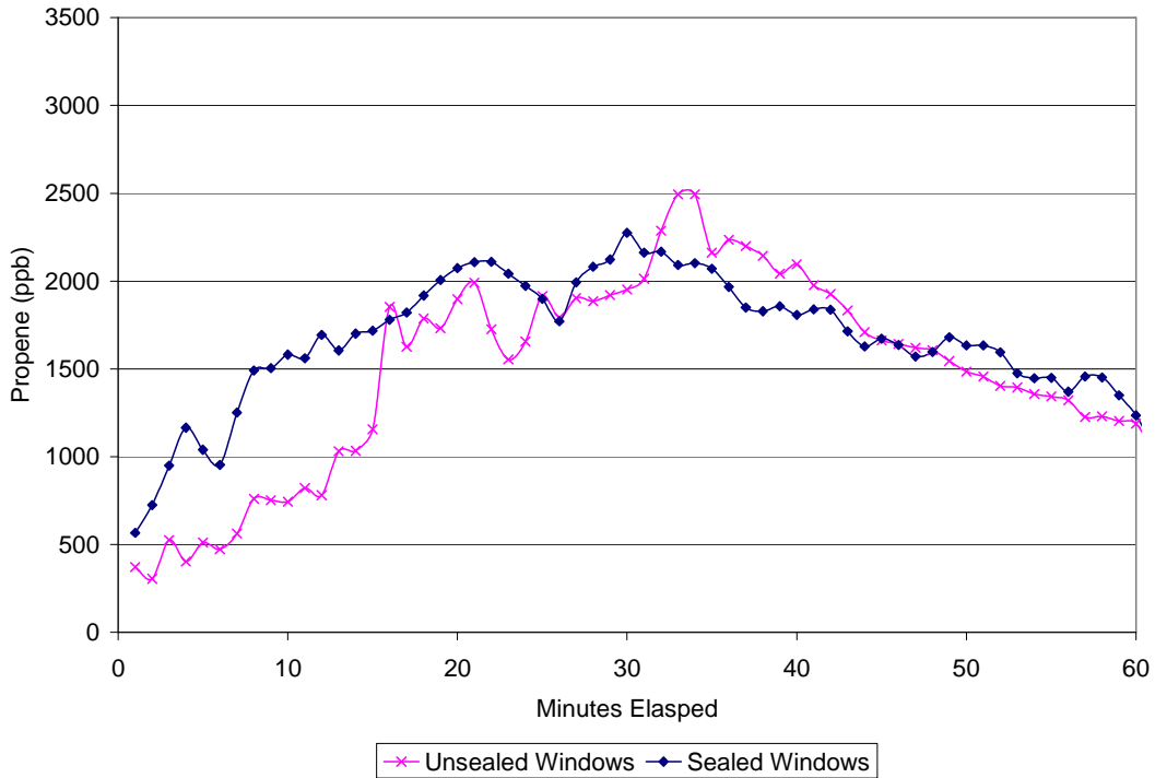
Figure 5.4.4.1 Average propene tracer gas concentrations (by exhaust position) in the bus cabin for windows sealed (0407) versus unsealed (0406).
