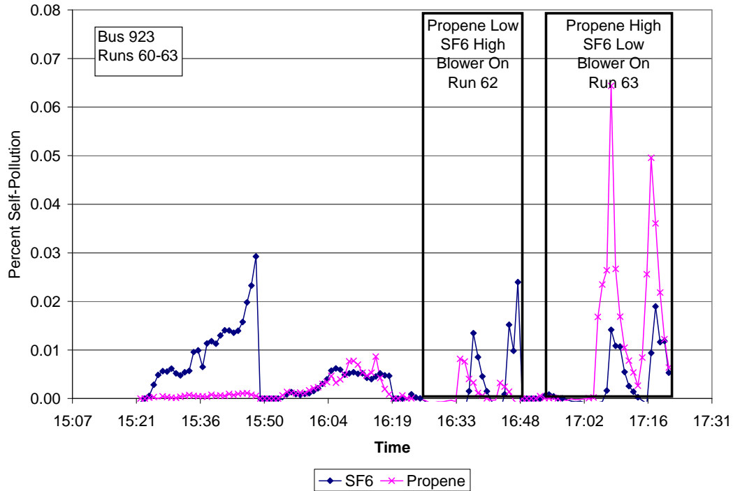
Figure 5.4.3.1.1 Time series of percent self-pollution for SF 6 and propene on 0510 examining the combination of exhaust position and blower operation as a mitigation measure.
